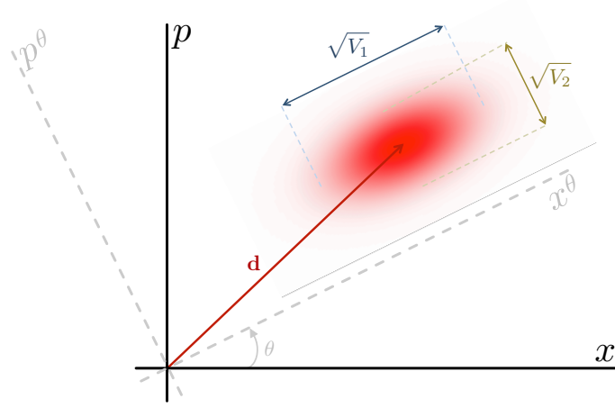
Figure 4. Wigner function of a generic Gaussian state (137). It consists of a single lob with the shape of an ellipse, centered at the position given by the mean vector \mathbf{d} . The covariance matrix V can be diagonalized through a rotation of angle \theta . Its eigenvalues provide the uncertainty of the quadratures along the principal axes of the ellipse.
